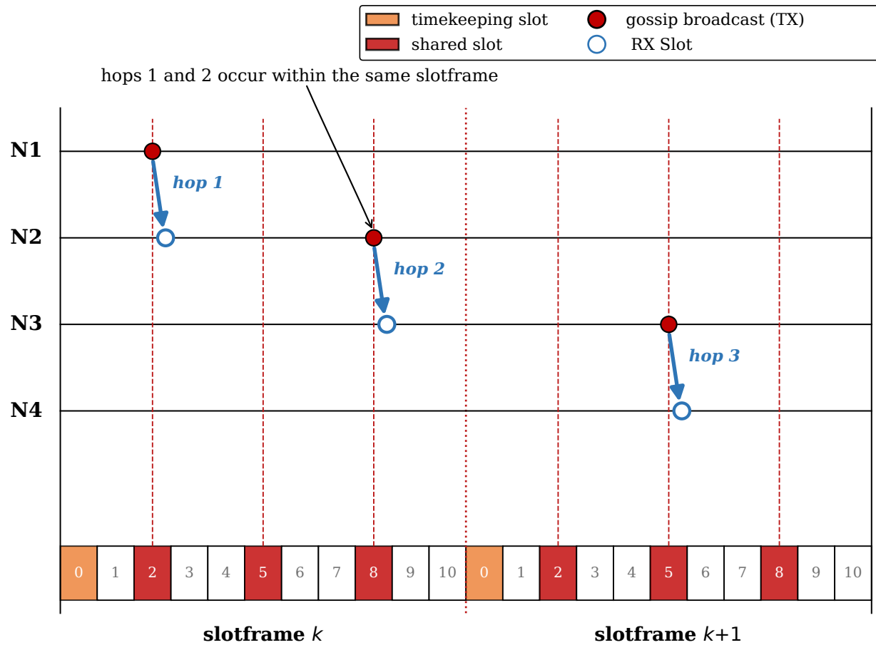
(b) Slotted propagation over TSCH
